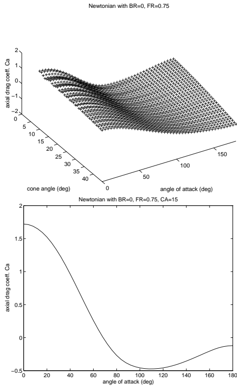
Figure 5. NEWTONIAN FLOW MODEL: C_a FOR VARIOUS \theta
