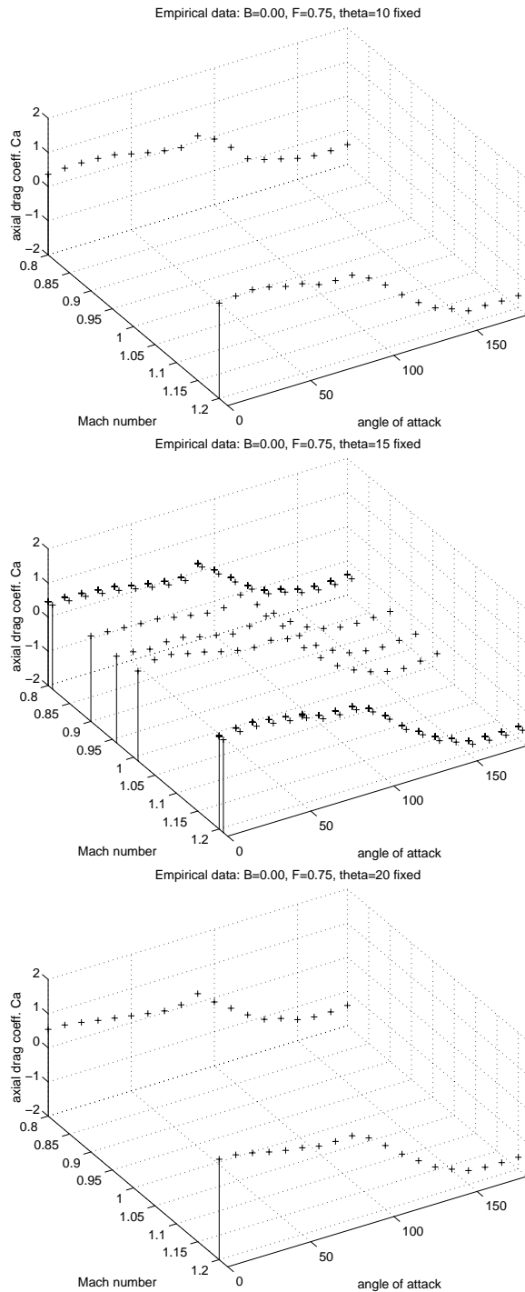
Figure 4. EMPIRICAL DATA: C_a FOR THREE CONE ANGLES \theta
