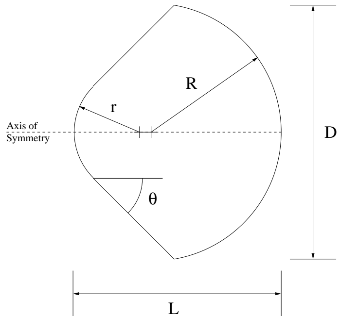
Figure 2. SCHEMATIC OF AEROSHELL
