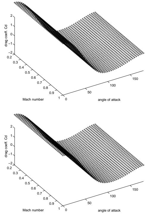
Figure 6. FREE-MOLECULAR FLOW MODEL: C_a FOR TWO \theta
