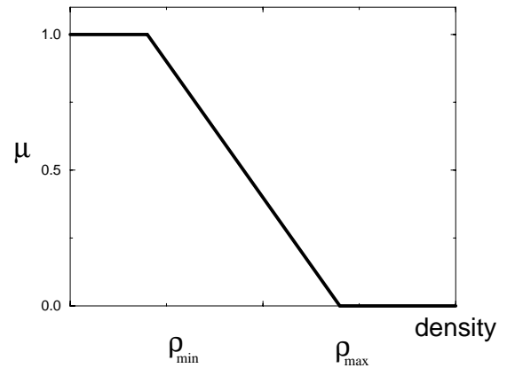
Figure 7. FUZZY SET EXPRESSING APPLICABILITY OF REGIME
